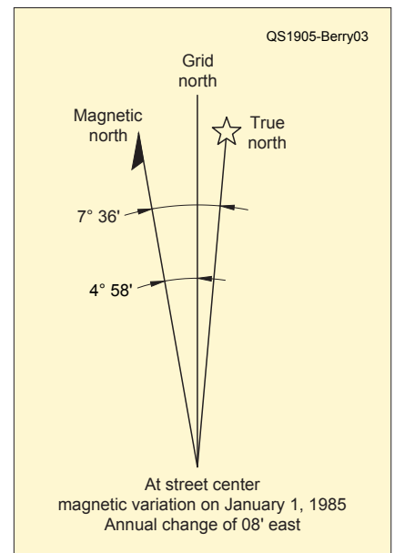
Figure 3 — Magnetic declination specification, generally located at the bottom of topographical maps.
