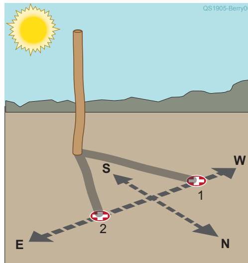
Figure 6 — Using the sun's shadow from a vertical pole to determine true north.
